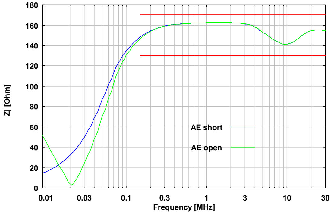
Impedanz an den Prüflingsklemmen - differential mode (Kalibrieradapter erforderlich), BNC mit 50 \Omega Abschluss Impedance at EuT-Terminals (Calibration adapter required), BNC-Port is terminated with 50 \Omega
