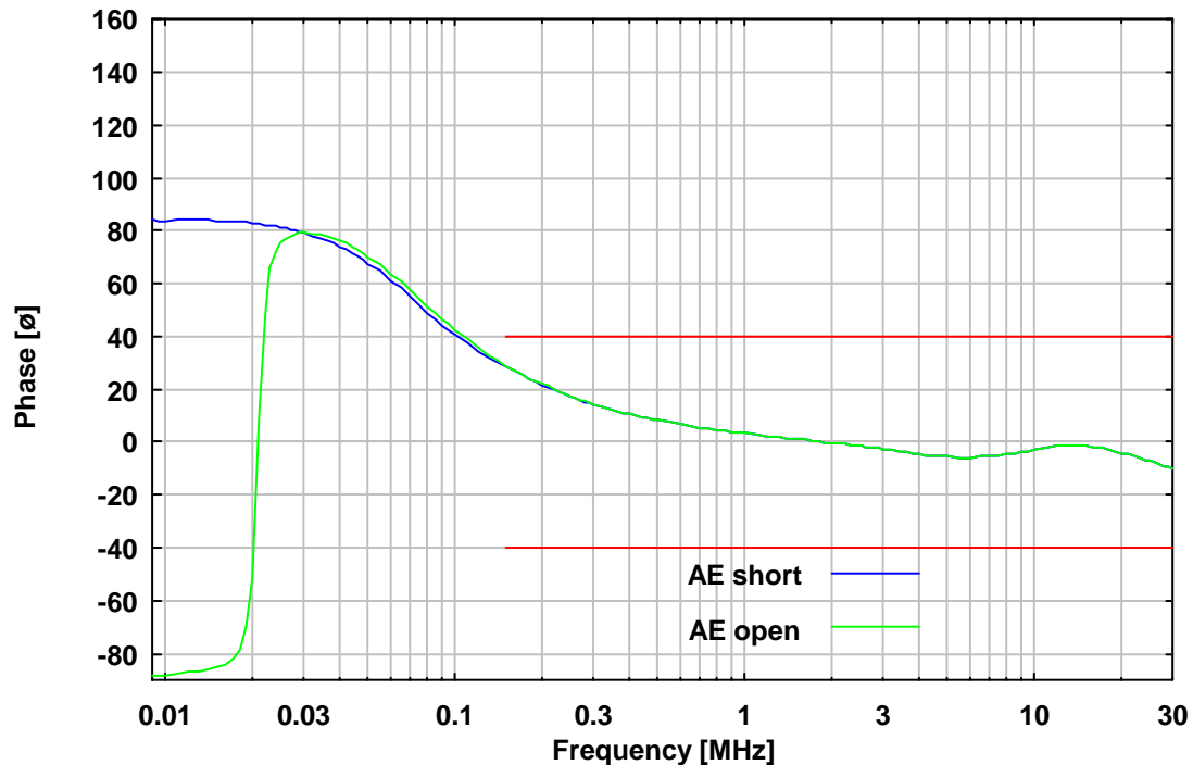
Phase an den Prüflingsklemmen - differential mode, (Kalibrieradapter erforderlich), BNC mit 50 \Omega Abschluss Phase at EuT-Terminals (Calibration adapter required), BNC-Port is terminated with 50 \Omega
